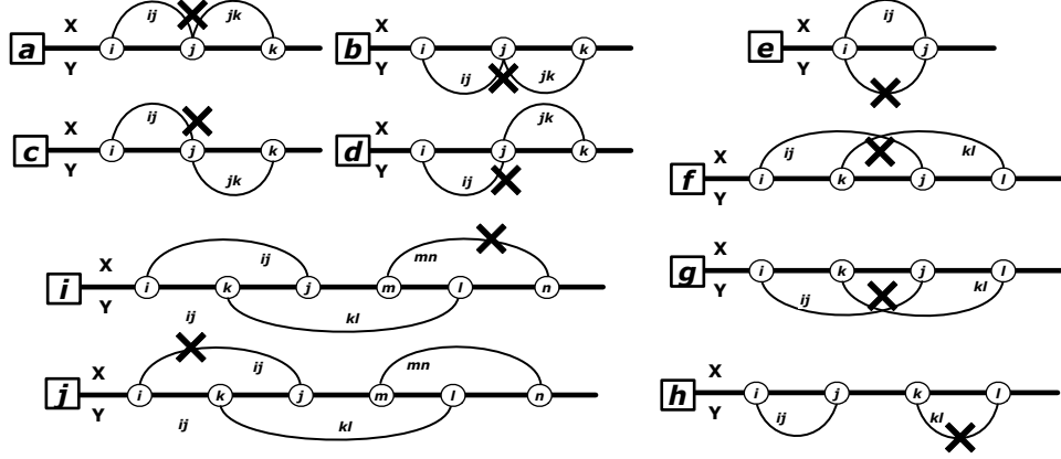
Fig. 1. RNA Constraints
