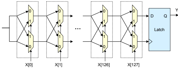
Figure 1: An arbiter PUF delay circuit. The circuit creates two input X , and produces an output Y based on which path is faster.
