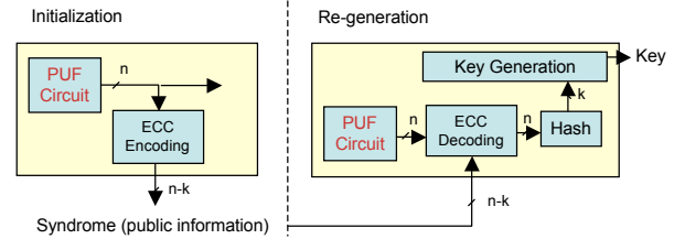
Figure 5: Cryptographic key generation with PUFs.
